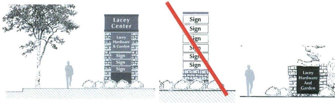
Figure 16.75.080(A)(4)(c-1). Illustrating acceptable and unacceptable freestanding sign examples. The left image utilizes a clearly identifiable top, middle, and bottom elements and meets the framing provision. The middle image includes a base, but insufficient top or framing element. The shorter sign to the right includes framing but is exempt from the top, middle, and bottom elements.
